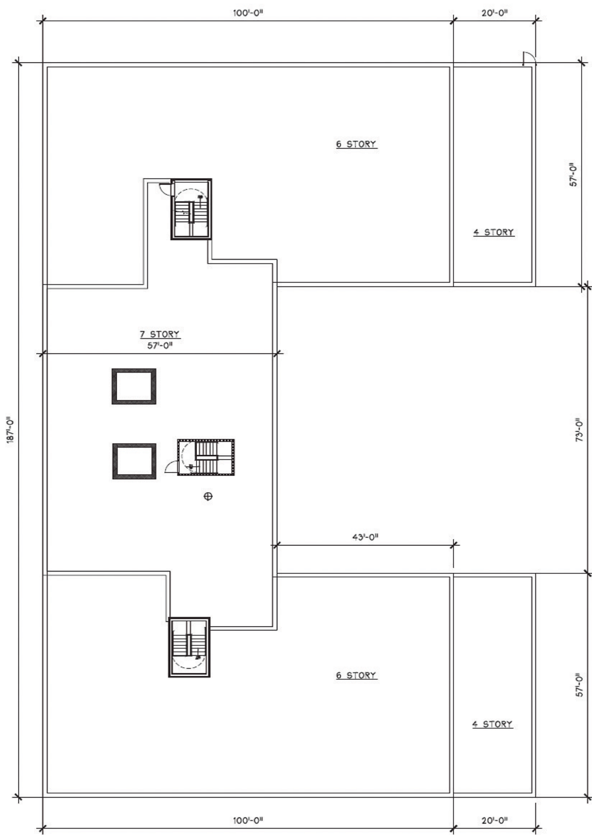
ROOF PLAN SCALE 1" = 20'-0"
