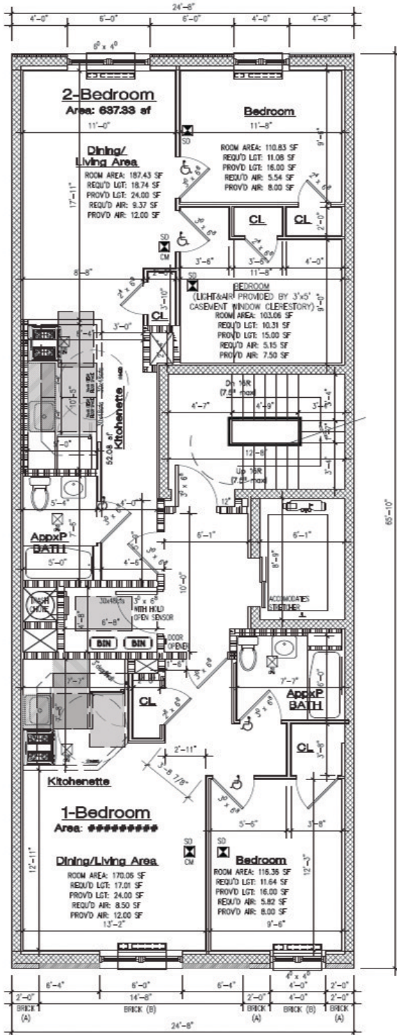
6th Floor Plan SCALE: 1/8"=1'-0"
