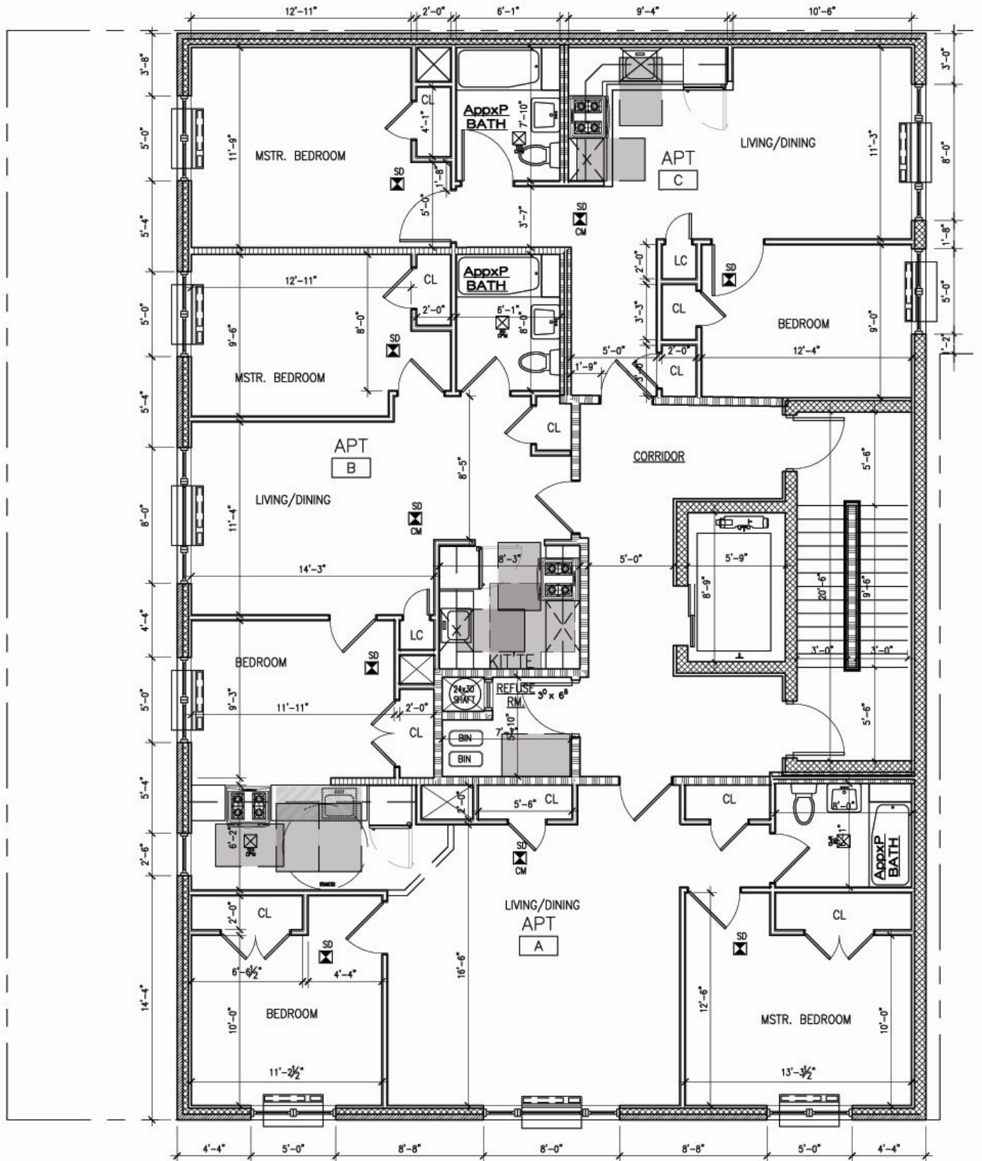
3rd THRU 5th FLOOR PLAN SCALE: 1/8" = 1'-0"
