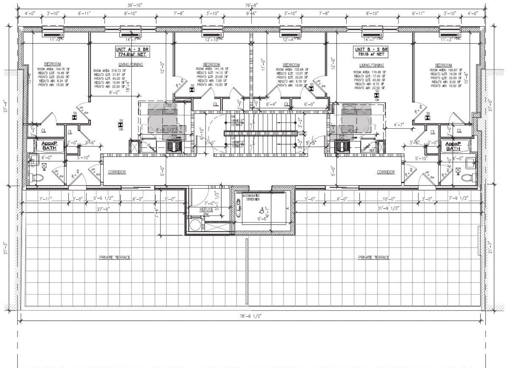
5TH FL. PLAN SCALE: 1/8" = 1'-0"
